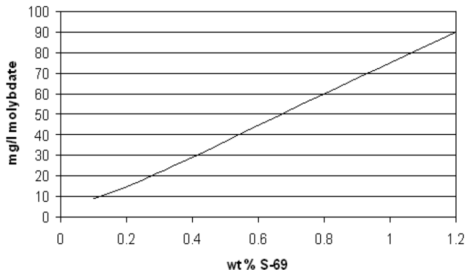
Approximate Concentration of Molybdate vs S-69
